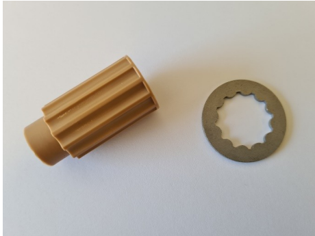
Standard feed roller with matching profile washer
